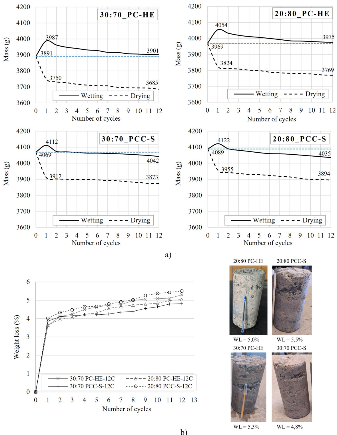
Figure 3. Mass variation (a) and weight loss (b) of specimens after W-D cycles.
