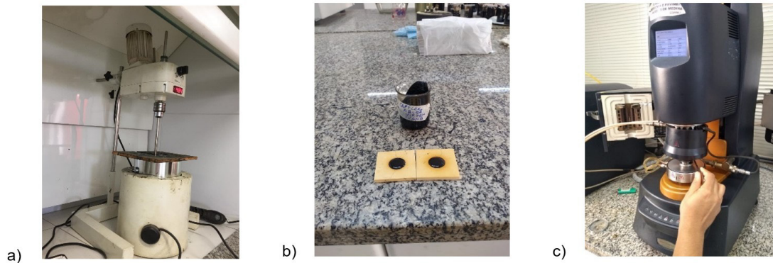
Figure 3. (a) Low shear stirring mixer with propeller, (b) 25 mm samples prepared and (c) dynamic shear rheometer
